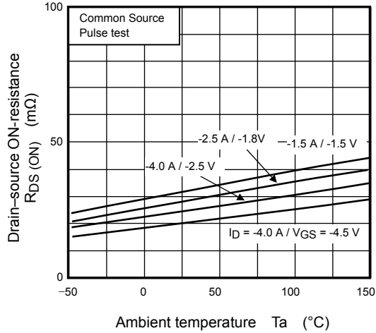
R_{DS(ON)} - T_a
